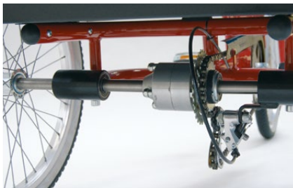
862 Three-speed gears with no backwards pedalling. Only sizes 3, 4, 5, 3D, 4D and 5D.
